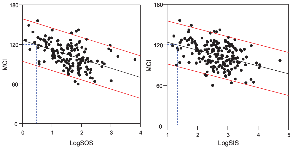
Figure 4-22. Linear relationships (with 95% prediction confidence intervals) between MCI and suspended organic sediment (n = 154), and suspended inorganic sediment (n = 183). Note that suspended sediment metrics are log-transformed. The blue line indicates the suspended sediment value where MCI exceeds 120.
