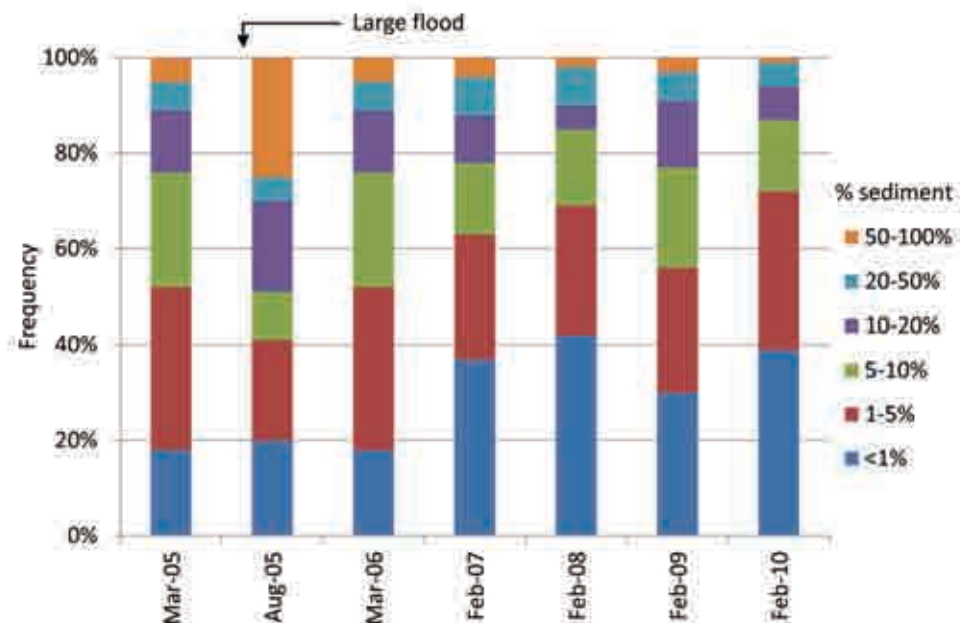
Figure 4-12. Temporal changes in % sediment cover in a run site on the Motueka River. A significant temporal trend was observed over a 5-yr period ( p = 0.003 ). Data courtesy of Les Basher, Landcare Research.
