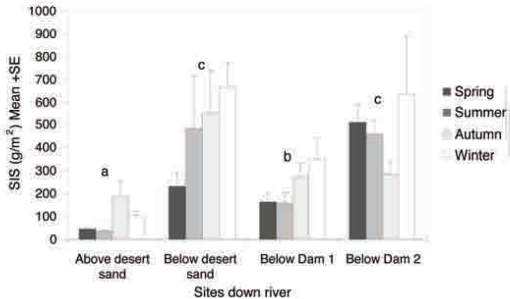
Figure 4-11. Seasonal patterns of Quorer suspended inorganic sediment ( \text{g/m}^2 ) in run habitat at sites down the Tongariro River in relation to the influences of sand input (from Rangipo Desert) and dams. Letters (above the bars) and lines (in seasons legend) indicate significant differences ( p < 0.05 ) using two-way ANOVA with Bonferroni post-hoc multiple comparisons (adapted from Quinn & Vickers 1992).
